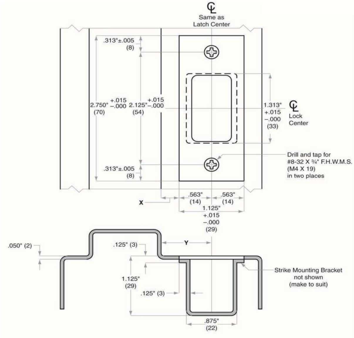
Dimensions X and Y are variables dependent on door thickness
